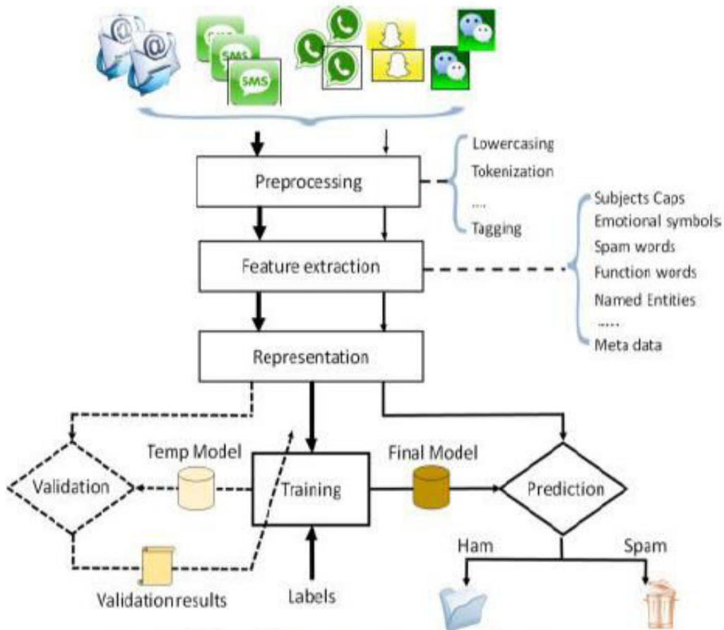
Fig 2: Flow Chart of SMS spam filtering [1]
