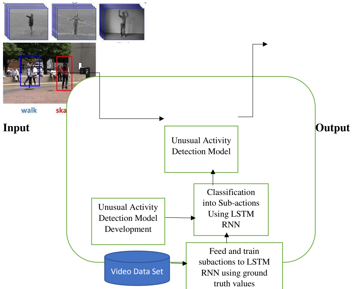
Figure1: Architecture Diagram for Unusual Activity & Anomaly Detection
